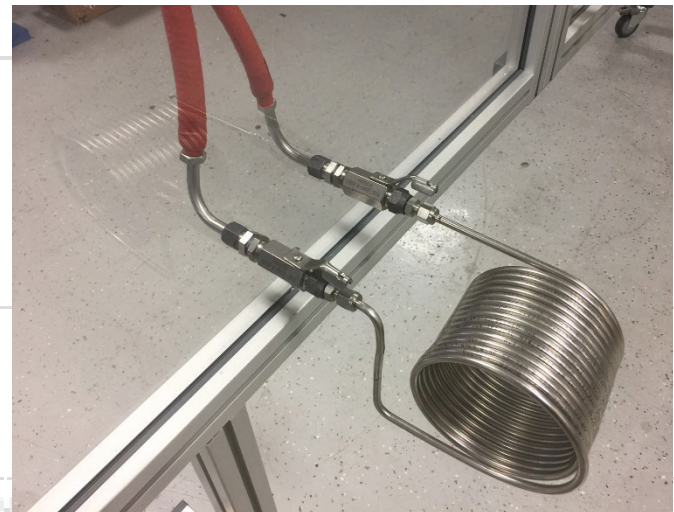
Pre-Constructed, cleaned and ready to install Restrictor Station to simulate pressure loss in an active station to keep the flow and pressure in balance in a paint circulation system.
