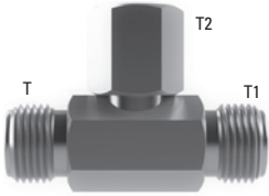
Male Straight X Male Straight X Female Tapered
