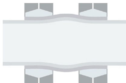
Pressed Condition (cross section)
